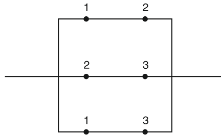
Figure 9.3 A two-out-of-three system.
